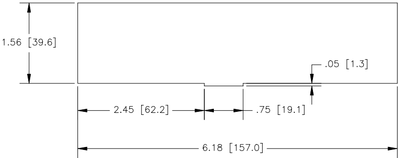
GTX 327 OLD RACK (115-00285-00)
