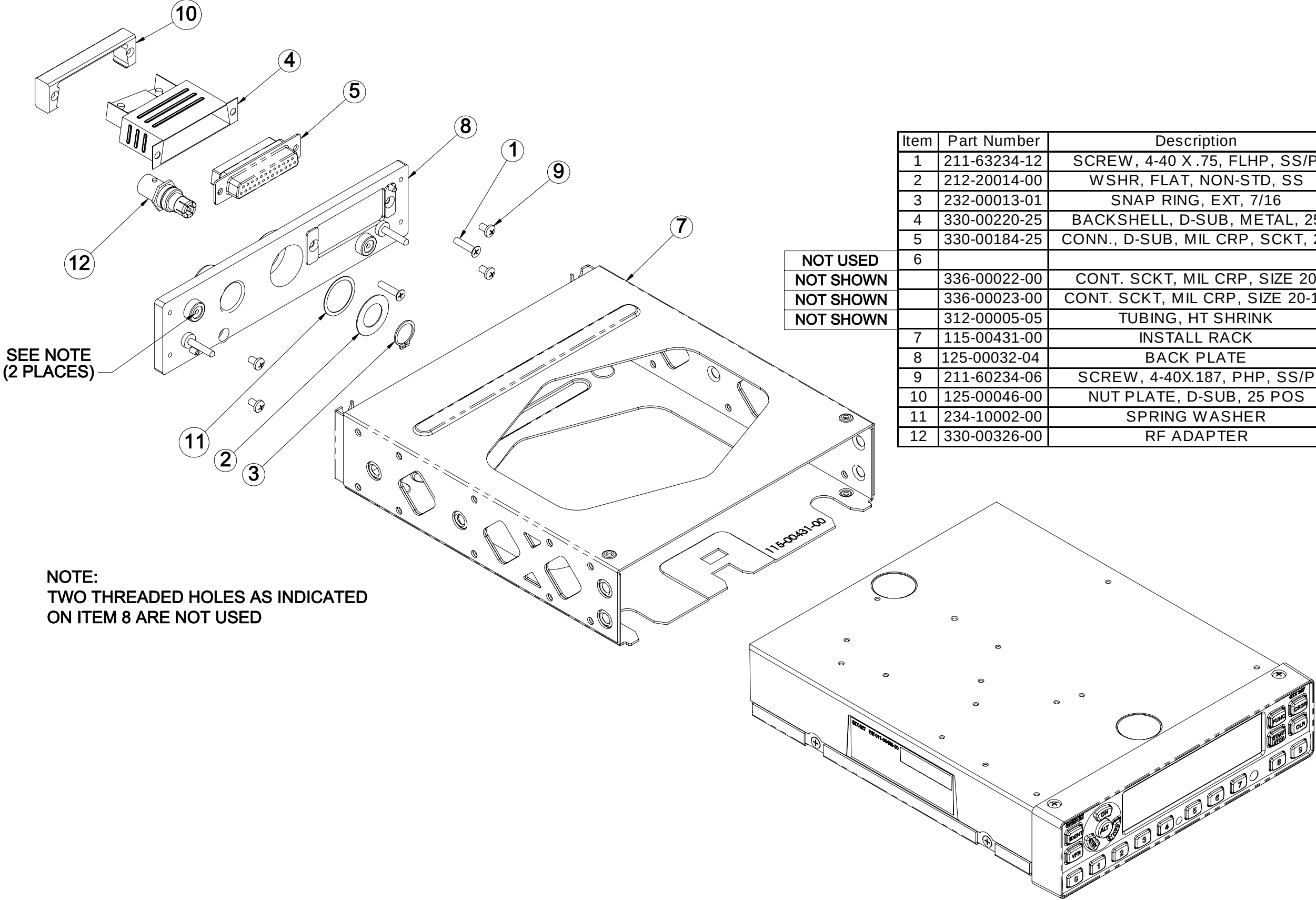
Figure B-2. GTX 327 Connector/Rack Assembly Drawing
