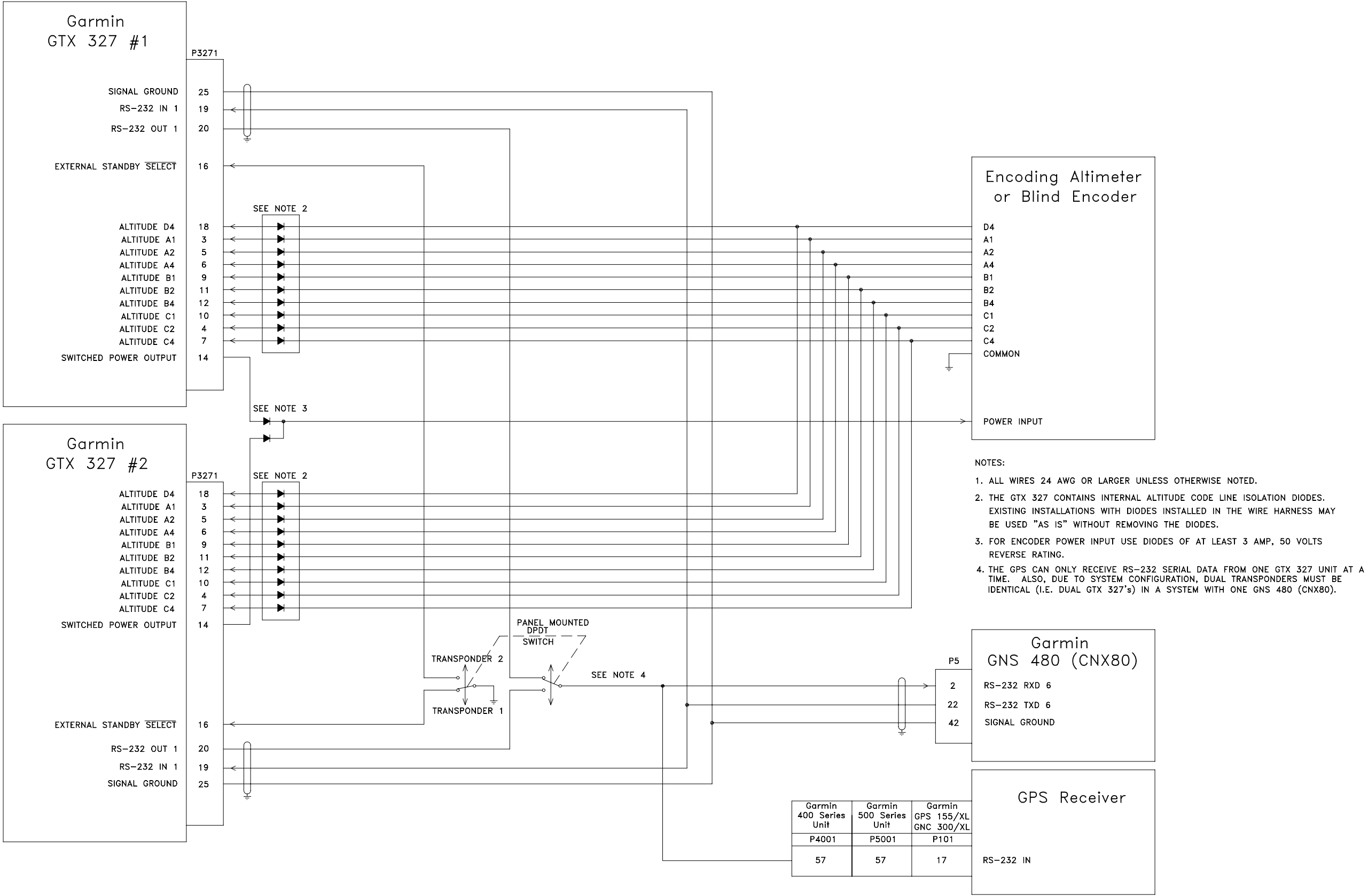
Figure C-4. Dual TXP Interconnect Wiring Diagram, Encoding Altitude Connections (Sheet 2)
