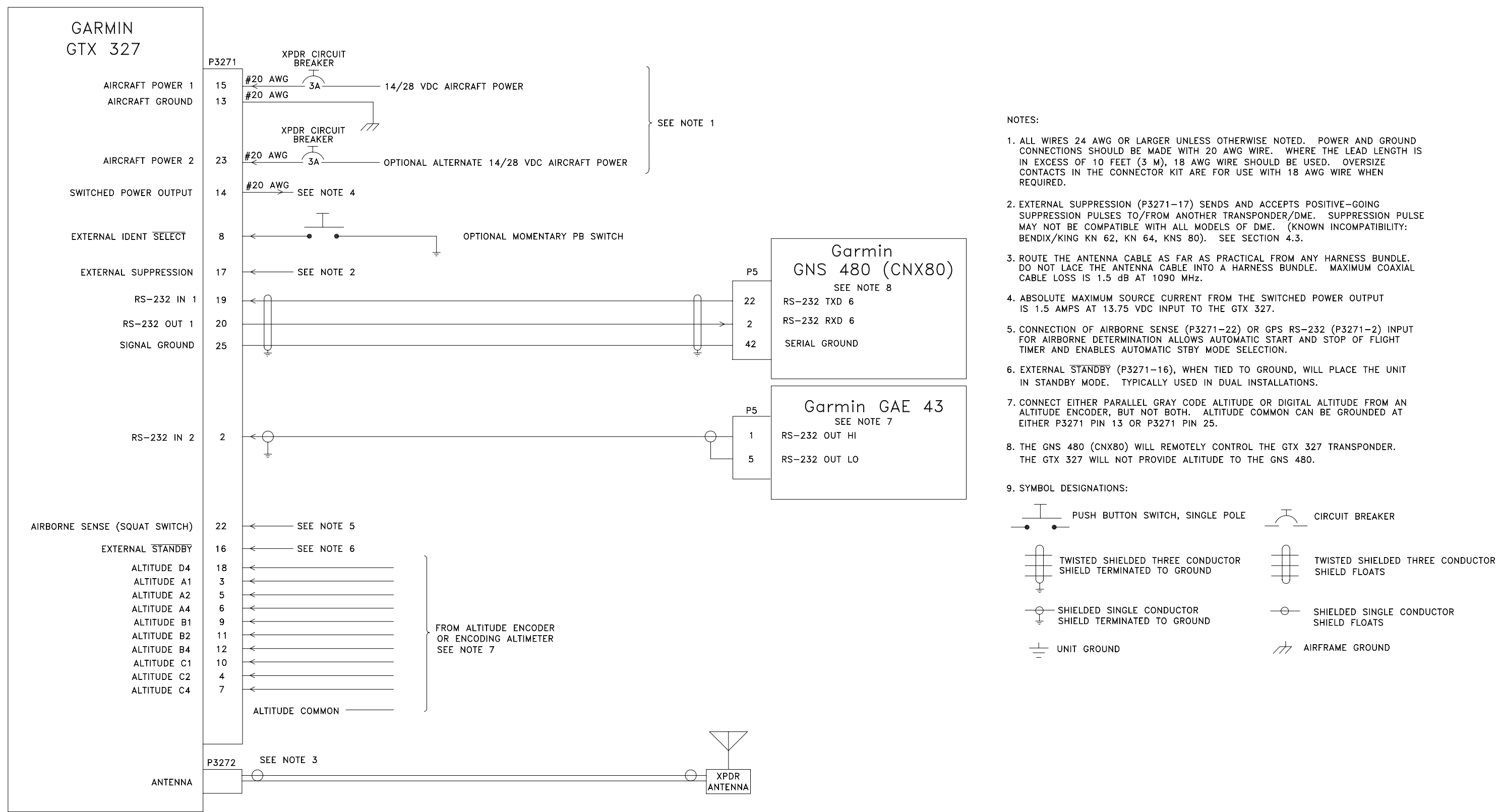
Figure C-2. GTX 327 to GNS 480 (CNX80), Typical Interconnect Wiring Diagram
